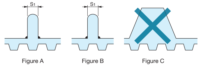
Maximum dimensions of profile mold width ( S_1 ) (mm)
